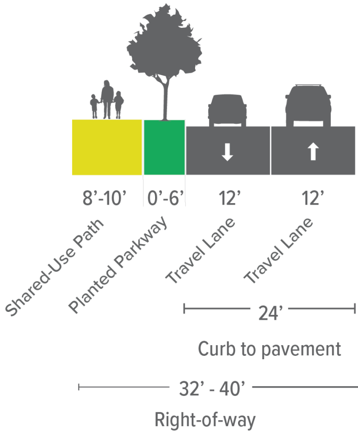
Figure 25 Cross-Section for Regional Thoroughfare
