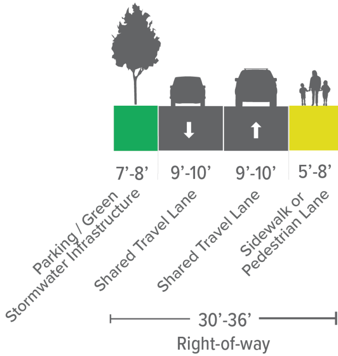
Figure 29 Cross-Section for Constrained Neighborhood Street
